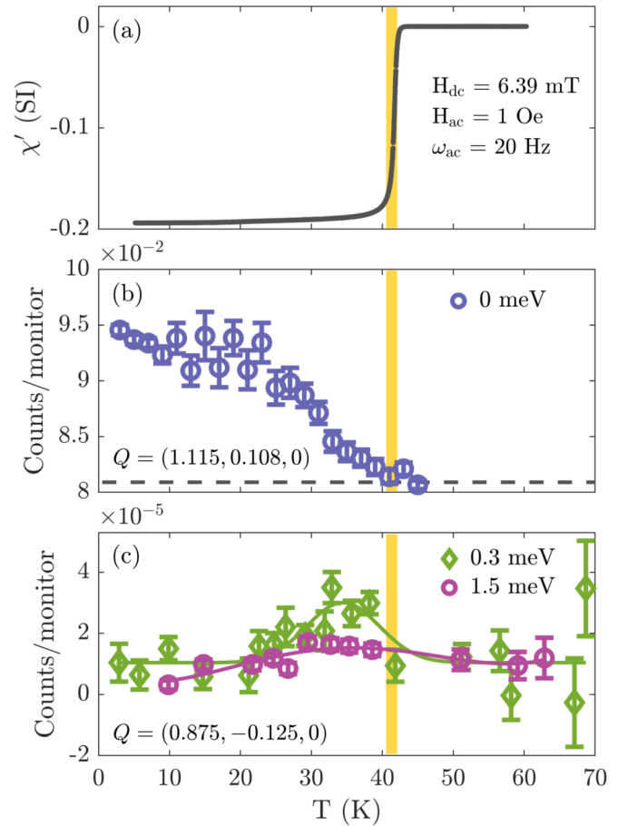
FIG. 1. (a) The real part of AC magnetic susceptibility, \chi' , showing the sharp transition to a diamagnetic state on cooling below the superconducting critical temperature. T_c is indicated by the yellow stripe which spans a temperature range 41.3 \pm 0.8 \text{ K} . The steps followed in the conversion from emu to SI units are presented in Appendix A. (b) Temperature dependence of magnetic order measured as 1-point scans on top of one of the IC peaks (1.115, 0.108, 0). The incoherent background has not been subtracted. The dashed line indicates the background level extracted from an energy scan away from the incommensurate peak position, at (1.1, -0.24, 0). (c) Temperature dependence of magnetic fluctuations with energy 0.3 and 1.5 meV. Data were measured as three-point scans with k_f = 1.2 \text{ \AA}^{-1} [ \Delta E = 0.070(1) \text{ meV} ] and the intensity is obtained as the difference between the point on top of the peak, at (0.875, -0.125, 0), and the average of the two background points.
