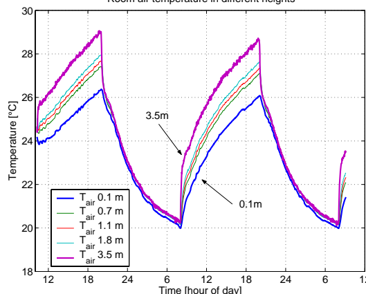
Room air temperature in different heights
