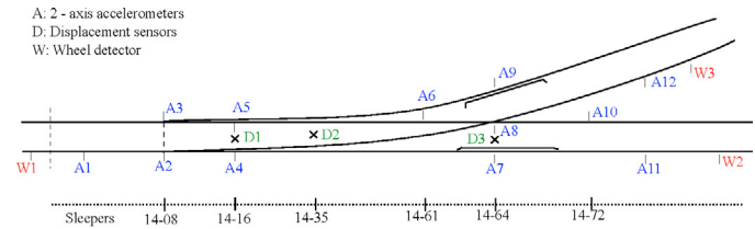
Fig. 1. Layout of the sensors location along the turnout at Tommerup station (Fyn - Denmark).
