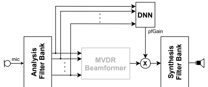
Fig. 2: Full system overview representing simplified internals of a HI. The highlighted parts (black) are used for the single-channel SE experiments.
