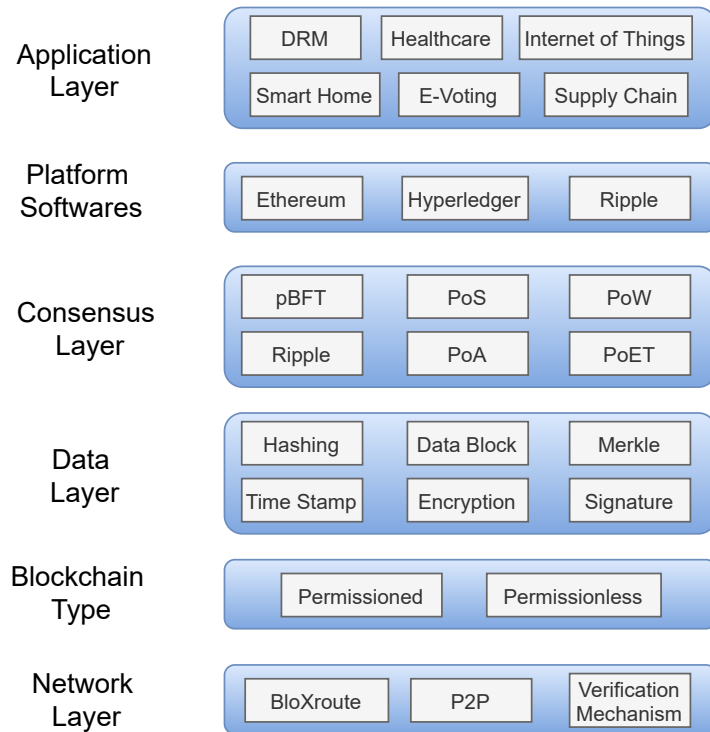
FIGURE 2 Blockchain Architecture.
