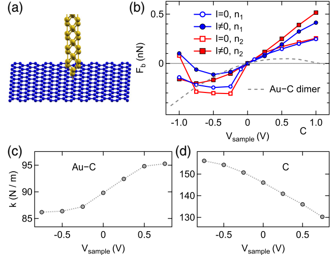
FIG. 3. (a) Model geometry comprising a quasi-one-dimensional Au tip and freestanding graphene. (b) Calculated bond force F_b(V_{\text{sample}}) [ F_b(0\text{V}) set to 0 \text{ nN} ] for the model geometry in (a) (solid lines) and a Au–C dimer (dashed line). The electric field is applied perpendicular to the graphene plane. Electron densities n_1 < n_2 are adjusted by the Dirac point energy, -400 \text{ meV} for n_1 and -700 \text{ meV} for n_2 . Solid (open) symbols reflect the presence (absence) of a current I . (c) Spring constant k_{\text{Au-C}} as a function of V_{\text{sample}} for doping n_1 . (d) Spring constant k_{\text{C}} as a function of V_{\text{sample}} calculated for displacing a C atom at doping n_1 .
