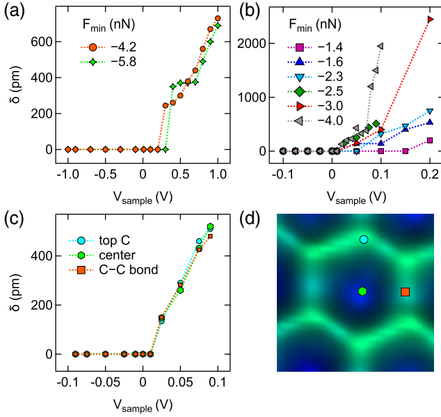
FIG. 2. (a) \delta(V_{\text{sample}}) for clean graphene. (b) Like (a) for Li-intercalated graphene. Different tips in (a) and (b) are characterized by F_{\text{min}} . (c) Site dependence of \delta(V_{\text{sample}}) for Li-intercalated graphene. (d) Constant-height \Delta f map [ 0.47 \times 0.47 \text{ nm}^2 , -8.7 (dark)– 7.5 Hz (bright)] of a graphene honeycomb cell.
