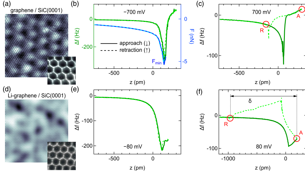
FIG. 1. (a) Constant-current STM image of clean graphene [bias voltage: -10 mV; tunneling current: 55 pA; size, 9.7 \times 9.7 nm 2 ; the gray scale ranges from 0 (black) to 67 pm (white)] with close-up view of the graphene lattice [ 1 mV, 33 pA, 0 (black)– 100 pm (white)]. (b) \Delta f(z) for clean graphene, V_{\text{sample}} = -700 mV (approach, from left to right, upper solid line; retraction, from right to left, upper dashed line). The vertical force F is displayed as the lower solid (approach) and dashed (retraction) line ( F_{\text{min}} , point of maximum attraction). (c) \Delta f(z) for clean graphene, V_{\text{sample}} = 700 mV (A, start of tip retraction; R, intersection of \Delta f_{\downarrow} and \Delta f_{\uparrow} data). (d) Like (a) for Li-intercalated graphene [ 100 mV, 51 pA, 10 \times 10 nm 2 , 0 (black)– 81 pm (white); close-up view, 100 mV, 50 pA, 0 (black)– 32 pm (white)]. (e) \Delta f(z) for Li-intercalated graphene, V_{\text{sample}} = -80 mV. (f) Like (e), V_{\text{sample}} = 80 mV. The loop width of \Delta f(z) is \delta . In (b),(c) and (e),(f), z = 0 pm is defined as the tip position prior to deactivating the feedback control and retracting the tip into the tunneling range ( z < 0 pm).
