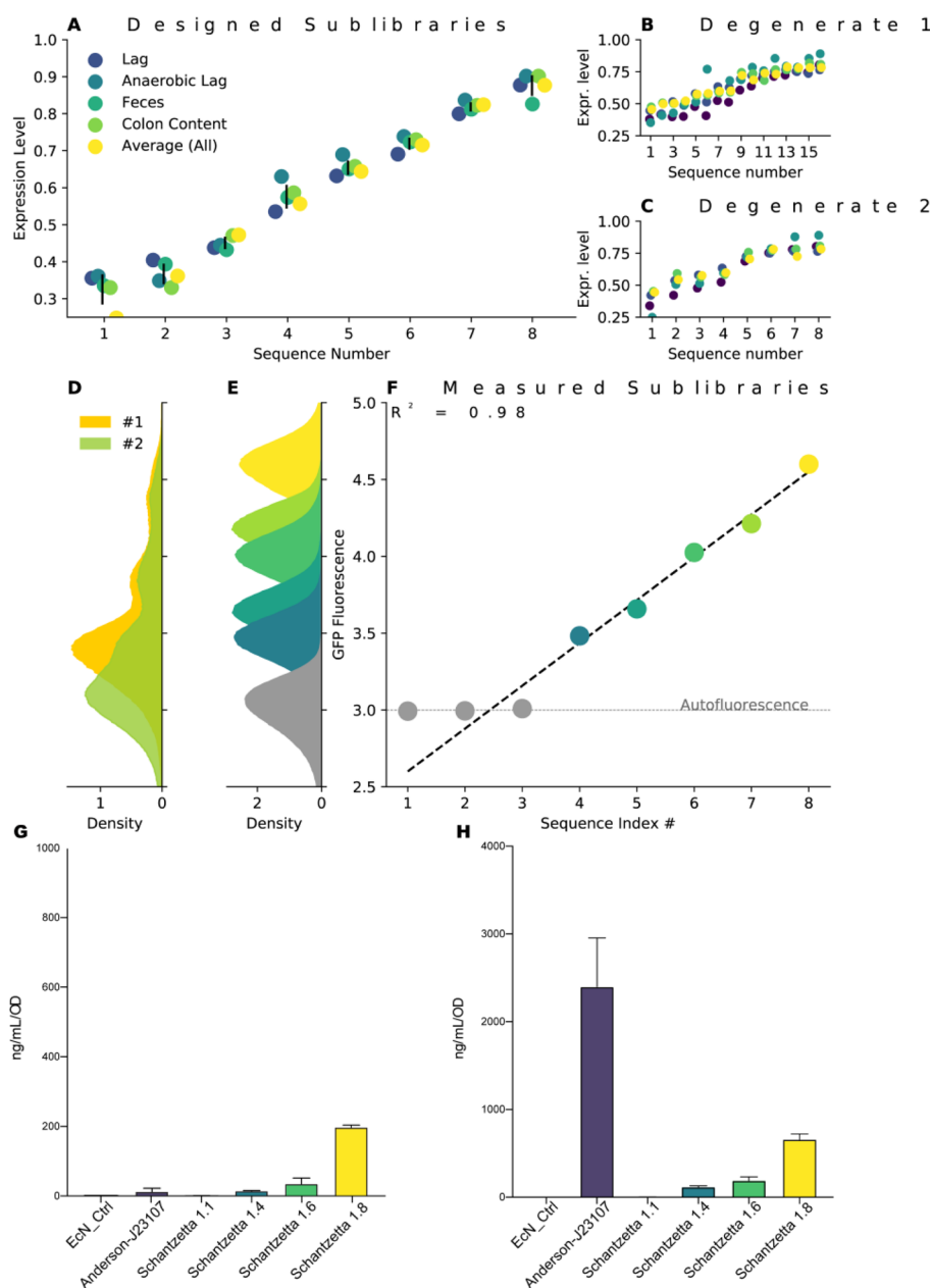
Figure 4. Determination of promoter libraries most suitable for predictable engineering across different environments. (A) Schantzetta library composed of eight promoter sequences with the highest degree of consistency between in vitro and in vivo environments. Chosen from lowest to highest with even spacing between them. Expression level is defined as in Figure 2B,C and compressed to the 0–1 scale. (B, C) Degenerate 1 and 2 sequences are determined in a similar fashion as the eight promoter sequences but must fit on a single degenerate primer for easy cloning. (D) Degenerate libraries re-cloned and measured in a flow cytometer in E. coli Nissle in the stationary phase, showing fluorescence at both low and high levels of expression. (E) Eight peaks of the individual promoter libraries measured in a flow cytometer in E. coli Nissle in the stationary phase. (F) Average expression of the eight individual promoter libraries compared with their sequence index. The three lowest expression levels show the same mean expression as the negative control, meaning that they do not show any expression above autofluorescence. The dashed line shows a linear regression of those promoter level measurements above negative control illustrating the high coefficient of determination ( R^2 = 0.98 , p value < 10^{-5} ). (G, H) In vitro expression in E. Coli Nissle of human hormones GLP1 (G) and IGF1 (H) under four promoters from the Schantzetta library (1.1, 1.4, 1.6, and 1.8). Expressions can be compared between a popular medium strength promoter from the Anderson library (J23107).
