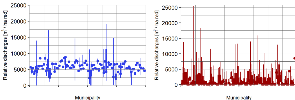
Figure 1. Reported relative discharges for separate systems (blue) and CSO (brown) for the 98 Danish municipalities.
