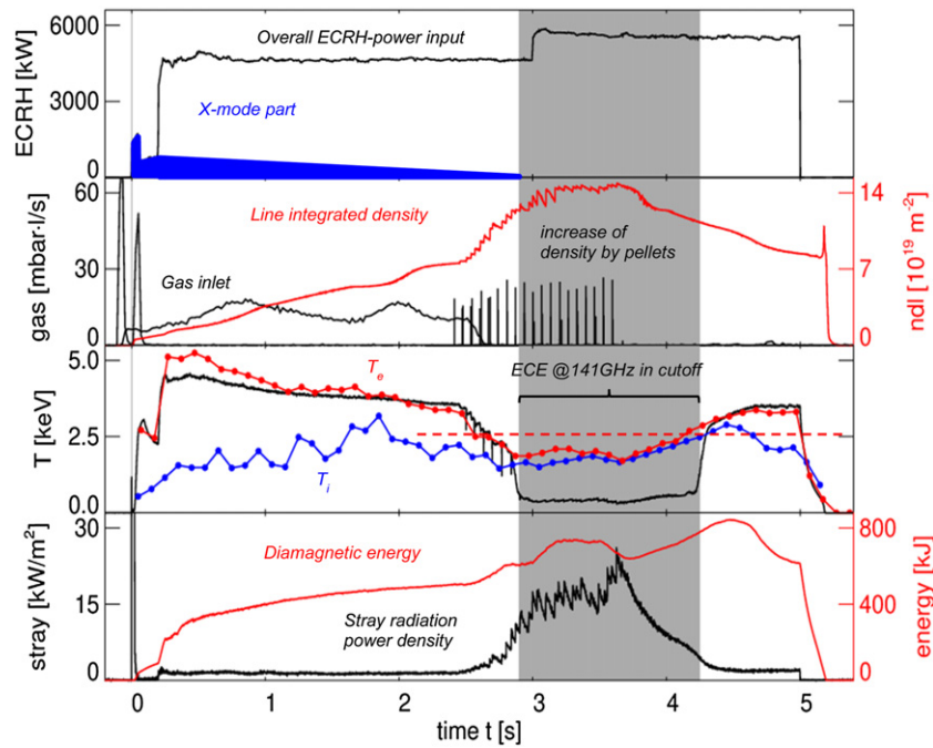
Figure 3. O2 ECRH scenario in combination with pellet injection (#20170904.015). For the plasma start-up three ECRH beams are polarized in X2-mode. During the density ramp their polarization is changed into O2-mode. The gray shaded area is the over-dense phase.
