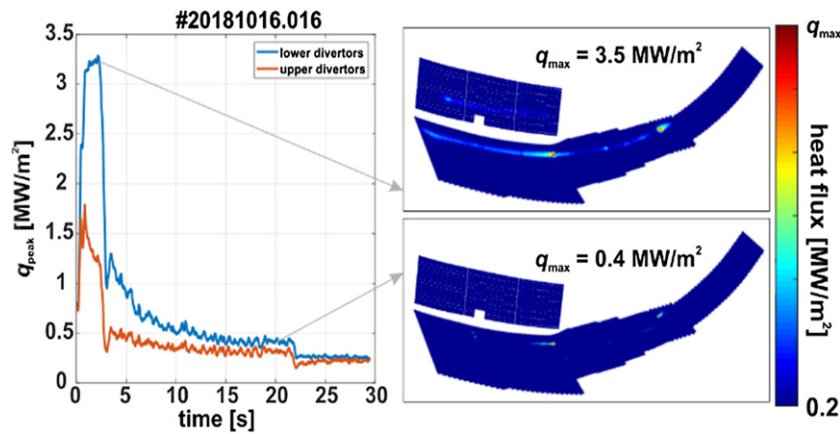
Figure 4. Left: time traces of the maximum heat flux at the divertor tile. Right: IR-picture of the divertor for attachment and detachment. Reproduced from [9].
