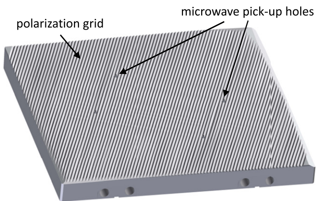
Figure 5. Tungsten covered TZM reflector tile with polarization grating on top.
