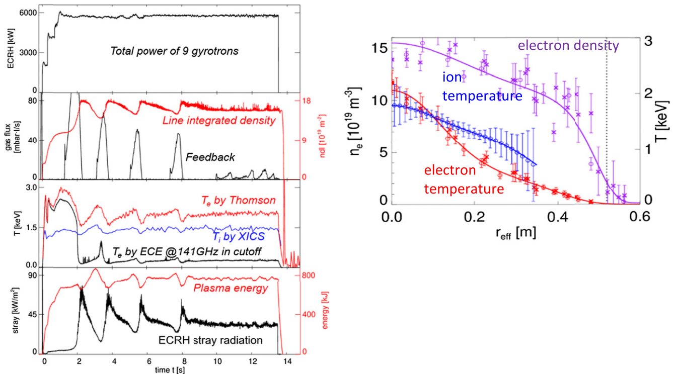
Figure 2. Left: time traces of a gas fuelled high density plasma with O2-ECRH only. Right: density and temperature profiles of the high density discharge.
