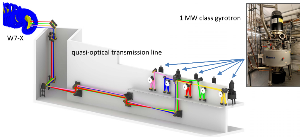
Figure 1. W7-X ECRH system. Here, one out of two models with five gyrotrons/beams is shown. The individual gyrotron beams, marked by different colours, are combined into a bundle and sent over a long distance with large common mirrors, the so called multi-beam section. They are divided into individual beams close to the vacuum vessel. Inside the vacuum vessel the beams are launched into the plasma by steerable mirrors.
