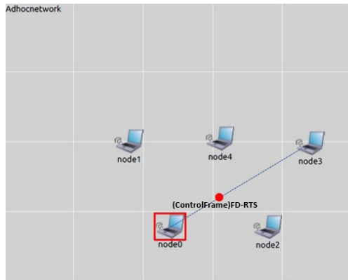
FIGURE 14. FD-RTS transmission from node0 to node3.
