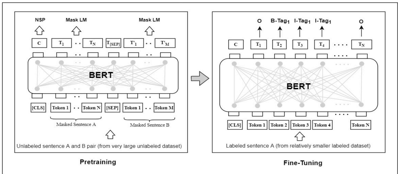
Figure 2. The pretraining and fine-tuning scheme for the BERT model. The same pretrained BERT model can be used for various natural language processing tasks.
