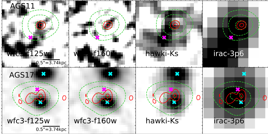
Fig. 4. Top: images of AGS11 in the J band, H band, K_s band and IRAC 3.6\mu\text{m} . The magenta “x” denotes the detection in K_s -band by ZFOURGE, \text{ID}_{\text{ZFOURGE}} = 7589 ( z_{\text{phot}} = 4.82 ). Bottom: same as above, but for AGS17. The cyan “x”s denote the optical bright neighbors, \text{ID}_{\text{CANDELS}} = 4414 ( z_{\text{phot}} = 0.03 , below) and \text{ID}_{\text{CANDELS}} = 4436 ( z_{\text{phot}} = 0.95 , above). The magenta “x” denotes the detection in K_s -band by ZFOURGE, \text{ID}_{\text{ZFOURGE}} = 6964 ( z_{\text{phot}} = 1.85 ).
