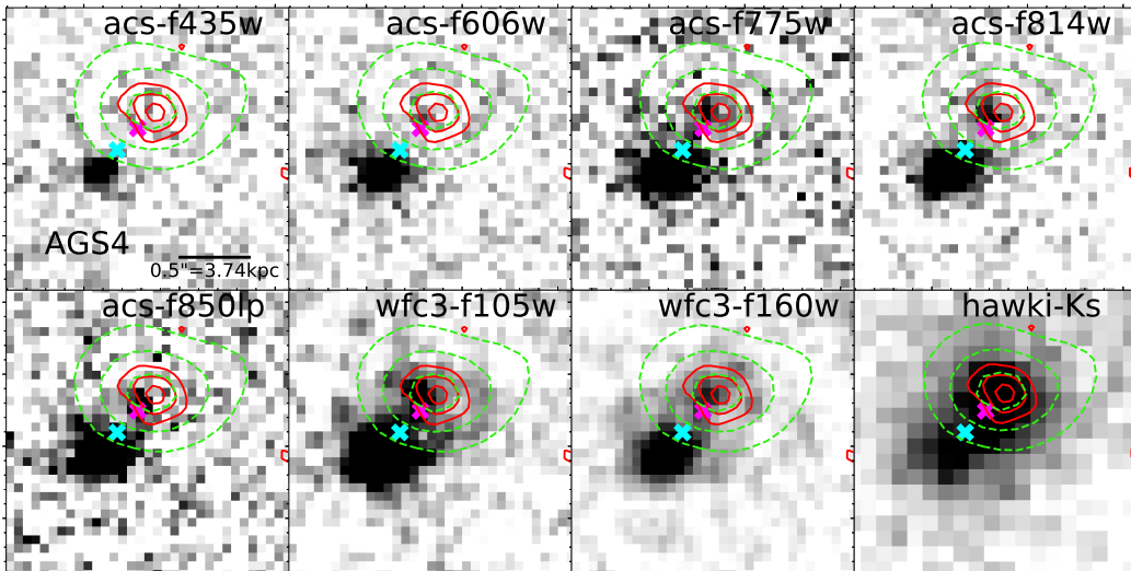
Fig. 6. Images of AGS4 from the observed B (435 nm, rest-frame UV) to near-infrared observed K_s ( 2.2 \mu\text{m} , rest-frame B ) bands. The red contours denote the ALMA detection at 1.1 mm at the resolution of 0''.29 . The green dashed contours denote the ALMA detection at 2 mm at the resolution of 0''.88 . The astrometric corrections between ALMA and HST images are applied throughout this work. The cyan “x” denotes the optical bright neighbor, \text{ID}_{\text{CANDELS}} = 8923 ( z_{\text{phot}} = 0.24 ). The magenta “x” denotes the detection by ZFOURGE based on the K_s -band image, \text{ID}_{\text{ZFOURGE}} = 12333 ( z_{\text{phot}} = 3.76 ). If not stated otherwise, the images in this paper are all oriented with the north up and east to the left.
