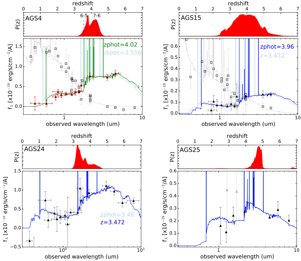
Fig. 2. Top-left: SED of AGS4. Top: photometric redshift PDF derived by EAZY (Brammer et al. 2008). Bottom: SED fittings. The green curve shows the best-fit of AGS4 at z_{\text{phot}} = 4.02 using EAZY, and we shift the SED to the spectroscopic redshift ( z_{\text{spec}} = 3.556 ) of AGS4 in light blue for comparison. The gray curve shows the SED of the optically bright neighbor, \text{ID}_{\text{ZFOURGE}} = 12333 . Top-right: SED of AGS15. The blue curve shows the best-fit at z_{\text{phot}} = 3.96 derived by EAZY and we shift the SED to the redshift peak of the overdensity, at z = 3.472 , in light blue for comparison. The gray curve shows the SED of the optically bright neighbor, \text{ID}_{\text{CANDELS}} = 3818 . Bottom-left: SED of AGS24. Same as AGS15. Bottom-right: SED of AGS25 at z_{\text{phot}} = 4.70 , fitted by EAZY with the photometry retrieved from the ZFOURGE catalog.
