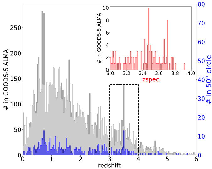
Fig. 8. Redshift distribution of the 11 674 galaxies with a redshift (either photometric or spectroscopic) located within the 6.9' \times 10' GOODS-ALMA field (gray). The subsample of 395 galaxies located within 50'' of the most massive galaxy AGS24, are shown in blue. The insert shows the distribution of the spectroscopic redshifts of the 121 galaxies at 3 \leq z_{\text{spec}} \leq 4 over the GOODS-ALMA field. Ten galaxies fall in the redshift bin 3.470 \leq z_{\text{spec}} \leq 3.480 . The mean redshift of the ten galaxies is z_{\text{spec}} = 3.472 . The redshifts are from the ZFOURGE (Straatman et al. 2016) and VANDELS DR3 (McLure et al. 2018; Pentericci et al. 2018) catalogs.
