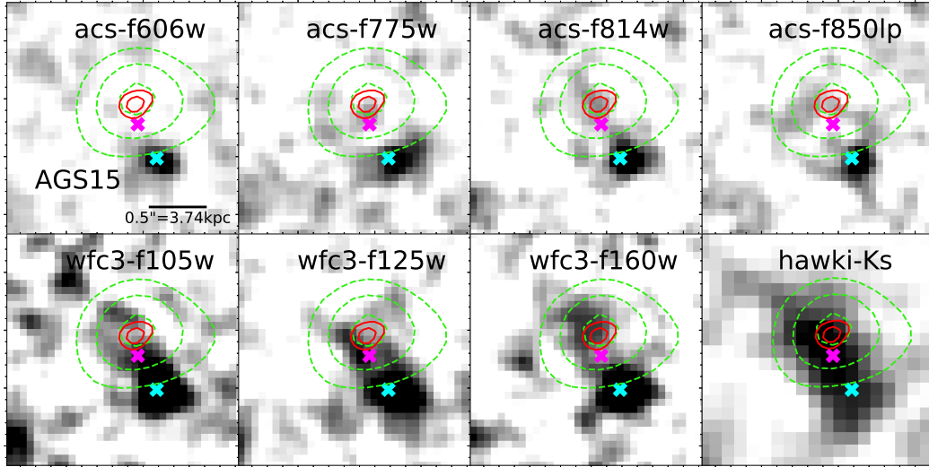
Fig. 9. Same as in Fig. 6, but for AGS15. The cyan “x” denotes the optical bright neighbor, ID CANDELS = 3818 ( z_{\text{phot}} = 4.27 ). The magenta “x” denotes the detection in K_s -band by ZFOURGE, ID ZFOURGE = 6755 ( z_{\text{phot}} = 3.47 ).
