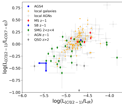
Fig. 3. Upper limit of the [CI](2-1)/CO(7-6) flux ratio of AGS4 (blue arrows), compared with existing observations of local and high-redshift MS galaxies, starburst galaxies and AGNs (data compiled in Valentino et al. 2018, 2020). If the detected emission line is indeed CO(7-6), then the flux ratio would fall at the lower end of the trend shown by the existing observations.
