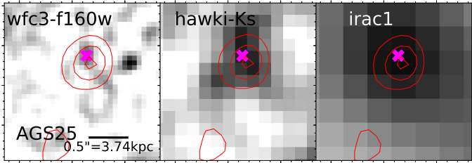
Fig. 7. Images of AGS25 in the H -band ( 1.6\ \mu\text{m} ), K_s -band ( 2.2\ \mu\text{m} ) and IRAC1-band ( 3.6\ \mu\text{m} ). The contribution of a 3'' distant bright neighbor of AGS25 was subtracted to produce the IRAC image as in F20a. The red contours denote the ALMA detection at 1.1\ \text{mm} at the resolution of 0''.60 . The magenta “x” is the ZFOURGE counterpart ID ZFOURGE = 11 353.
