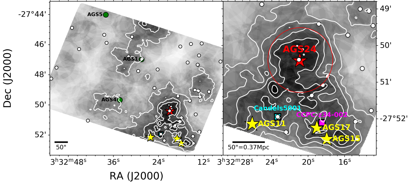
Fig. 10. Projected density of 364 galaxies (40 with z_{\text{spec}} ) at 3.42 \leq z \leq 3.57 . The contours show 1, 2, 3, 4\sigma level of the overdensity. Left panel: field observed in GOODS-South ALMA. Right panel: zoom-in of the extended structure in the bottom right corner of GOODS-ALMA field that encompasses 126(18) galaxies over 15 \text{ arcmin}^2 . The red star indicates the position of AGS24. The red circle indicates a 50'' radius region ( 2 \text{ arcmin}^2 ) including 26(3) galaxies. The yellow stars refer to the HST-galaxies AGS 11, 15 and 17 located also in this larger structure. The green circles represent the AGS 1 and 5, which are also in this redshift range but not optically dark. The white circles show the 40 galaxies with spectroscopic redshifts. We note that the two white circles falling on the red star of AGS24 are two galaxies dissociated from AGS24. The magenta square denotes the center of the proto-cluster CCPC-z34-002 identified by Franck & McGaugh (2016). The cyan square denotes CandelS5001, which used to be the most massive galaxy at 3 < z < 4 in this field (Ginolfi et al. 2017). The 50'' scale in the figure is equivalent to a proper distance of 0.37 Mpc at z = 3.5 .
