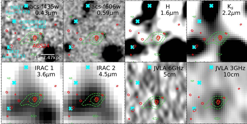
Fig. 5. Images of AGS24 in the B , V , H and K_s band, IRAC 3.6 and 4.5 \mu\text{m} , JVLA 6 GHz ( 3.7\sigma ) and 3 GHz ( 5.7\sigma ). The contours are the same as in Fig. 6 but for AGS24. The three neighbor galaxies are labeled with \text{ID}_{\text{ZFOURGE}} or \text{ID}_{\text{CDFS}} and their redshift separately.
