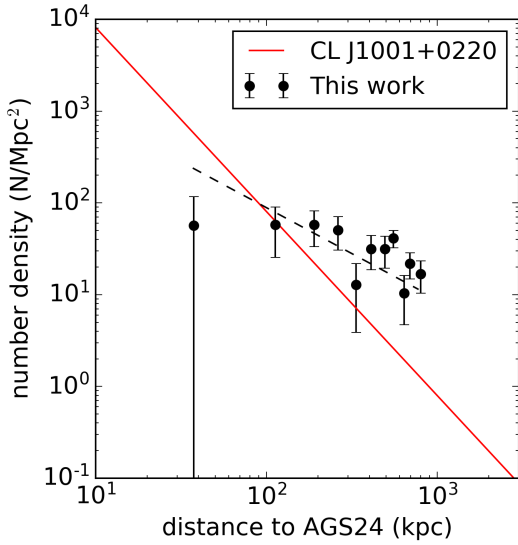
Fig. 13. Projected numbers of galaxies in the overdensity as a function of their distance to AGS24 (black circles) and the black dashed line is the linear fitting to the profile. The red line shows the best-fit projected NFW profile (Navarro et al. 1996) of a galaxy cluster at z = 2.506 , CL J1001+0220 (Wang et al. 2016).
