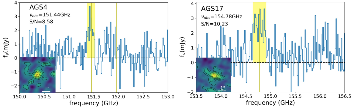
Fig. 1. Left: part of the spectrum obtained from the ALMA band 4 observation of AGS4. The yellow shade highlights the detected emission line. The emission line map is shown in the bottom-left corner. The contours denote 1 to 5\sigma , with the step of 1\sigma . Right: same as on the left, but for AGS17. The contours in the map denote 1 to 6\sigma , with the step of 1\sigma .
