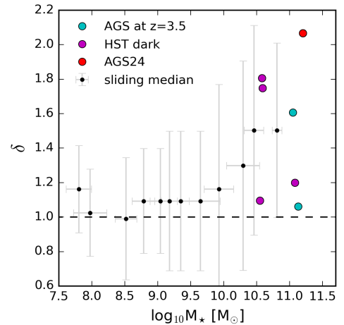
Fig. 11. Local overdensity ( \delta ) of individual galaxies in the GOODS-ALMA field at 3.42 < z < 3.57 . The black dots show the sliding medians of \delta at different stellar masses. The filled circles indicate all the ALMA detections. The purple circles are the HST dark galaxies and the red circle indicates AGS24.
