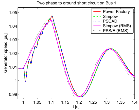
Fig. 12 Generator speed during the second 2-phase to ground short circuit
