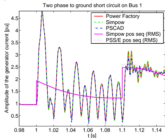
Fig. 9 Generator current during the first 2-phase to ground short circuit
