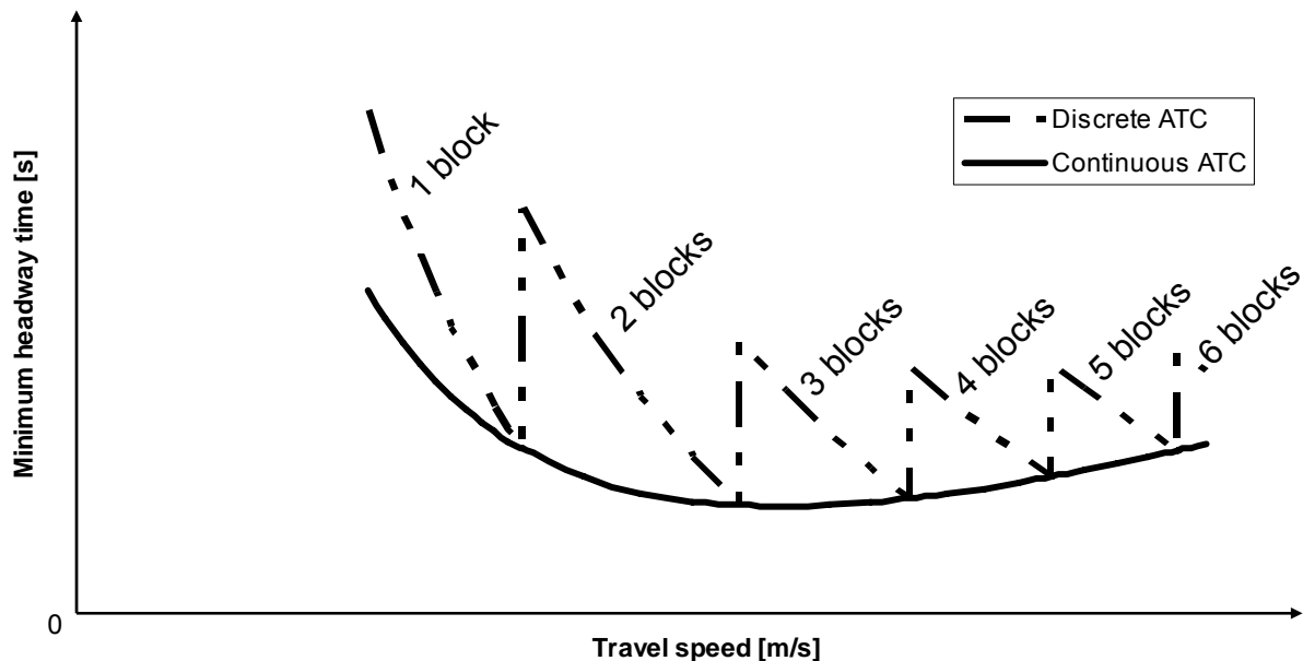
Figure 10: Minimum headway time (for traditional block systems) according to the speed of the train [13].
