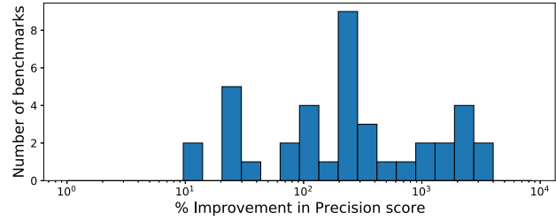
Figure 11: Histogram of Percentage Improvement in Precision scores for individual programs.
