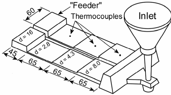
Fig. 3 Casting layout
