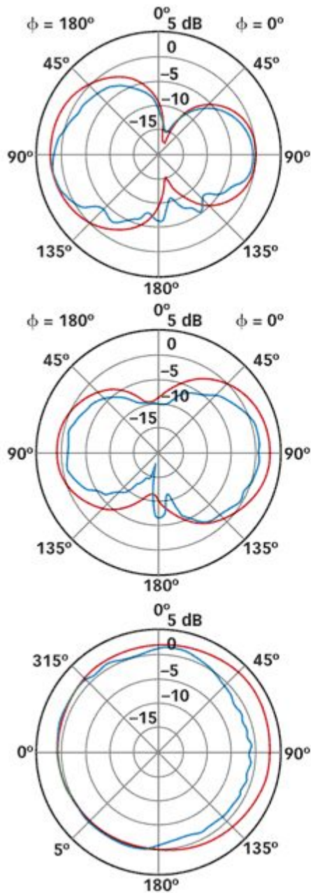
6. These plots show the simulated (solid) and measured (dashed) total electrical field components of the radiation pattern, \theta -cuts for \Phi = 0^\circ (a) and for \Phi = 90^\circ (b), and \theta -cut for \Phi = 90^\circ (c) the 40-mm-long capacitor loaded PIFA.
