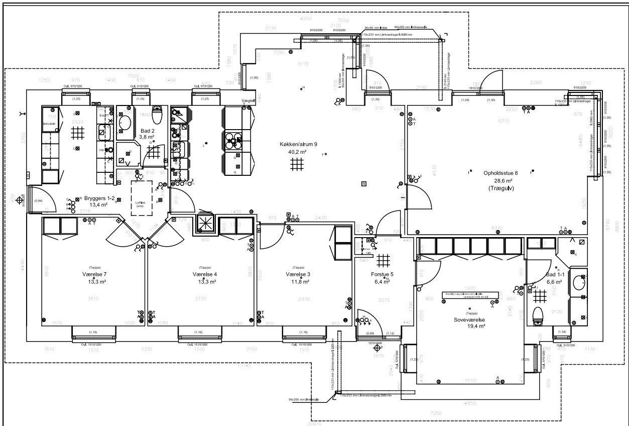
Figur 10. Plantegning.
