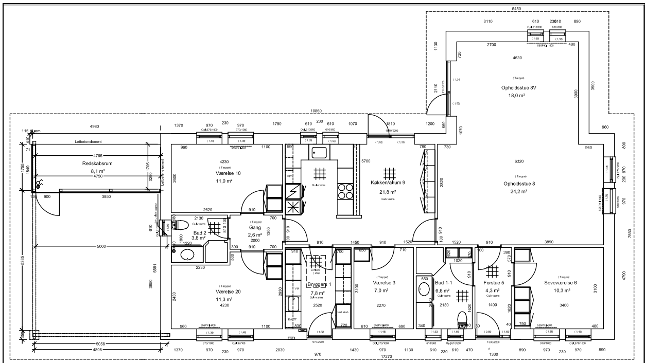
Figur 2. Plantegning.
