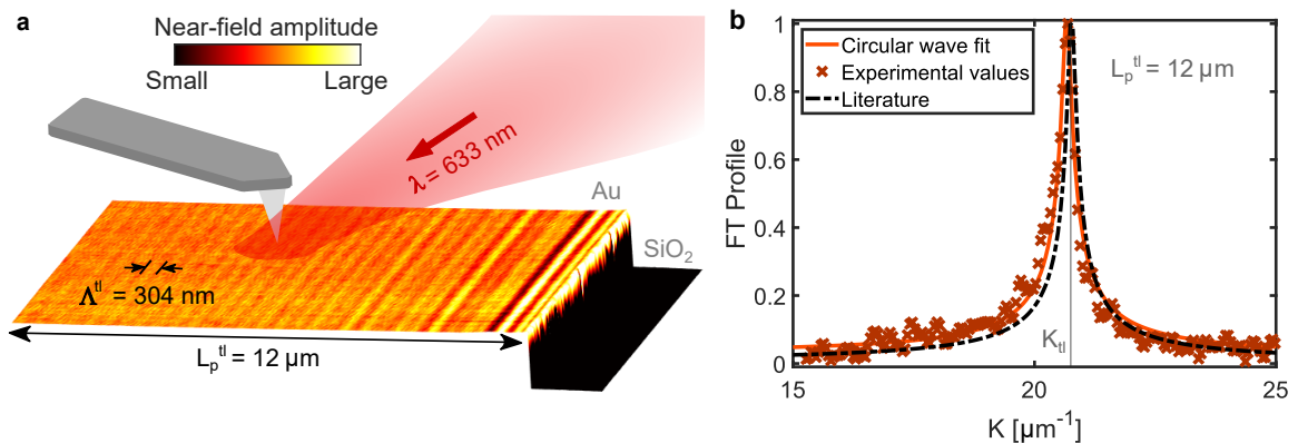
Fig. 1: Experimental details and main result. (a) Simplified schematic of the s-SNOM measurement. The near-field amplitude from one of our measurements is shown on the gold surface. \Lambda^{\parallel} is the SPP wavelength and L_p^{\parallel} is the propagation length. (b) Fourier transform of the profile extracted from the near-field amplitude displayed in (a). K_{\parallel} is the SPP wavevector
