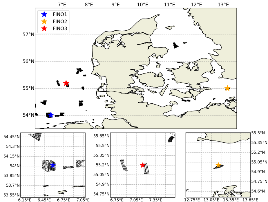
Figure 1. Map of the study area with the FINO mast locations in the North Sea and Baltic Sea (top). The black shapes represent nearby offshore wind farms. The bottom panels show close-ups for the met mast locations with black dots representing individual wind turbines.
