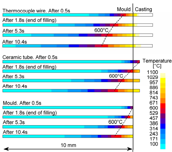
Fig. 6 Temperature difference between surface of TC and CC3-6, from simulation 4 (8 mm plate)
