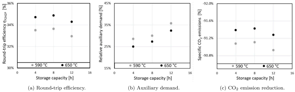
Fig. 7. Evaluation of three main technical parameters for all cases considered in this work.
