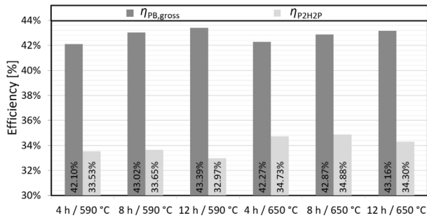
Fig. 8. Comparison of annual efficiencies.
