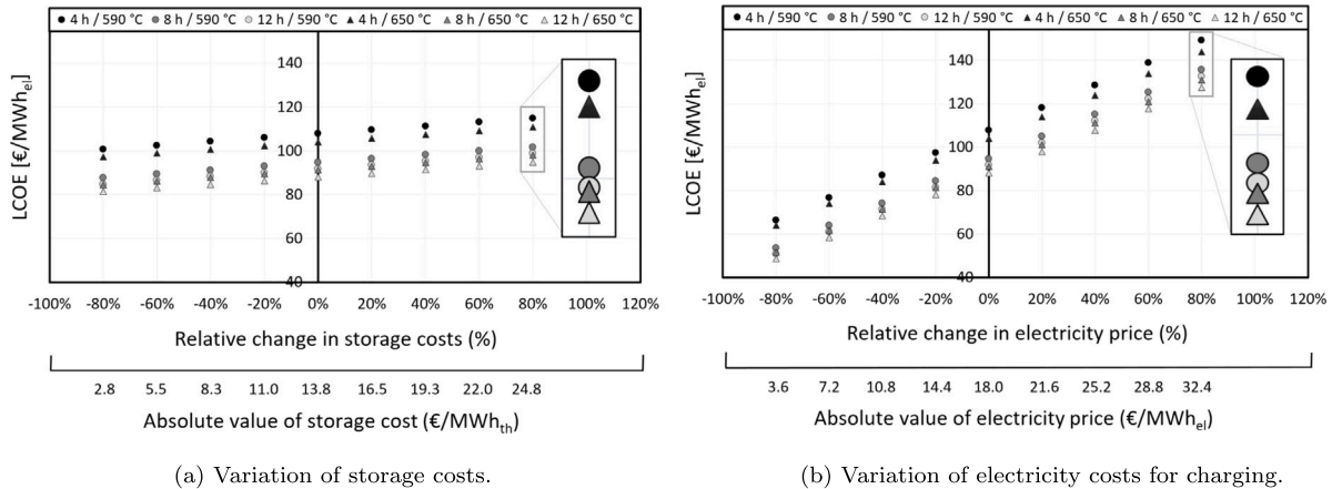
Fig. 11. Sensitivity analysis of LCOE. Please note that absolute LCOE values are plotted on the ordinate.
