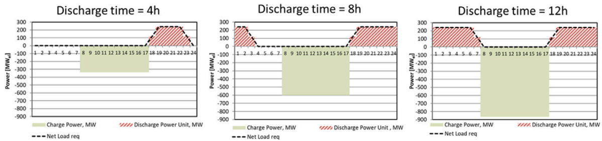
Fig. 4. Daily operation profiles for the cases studied (Table 3): 300-MW plant, 10-h charging duration and discharging duration of 4 h, 8 h and 12 h.
