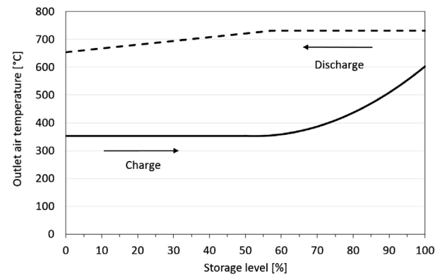
Fig. 3. Characteristic storage outlet air temperature during charge and discharge. No cyclic effects considered, valid for all boundary conditions used in this study. The storage level is defined as the ratio between the actual stored energy and the maximum thermal capacity from Eq. (3).
