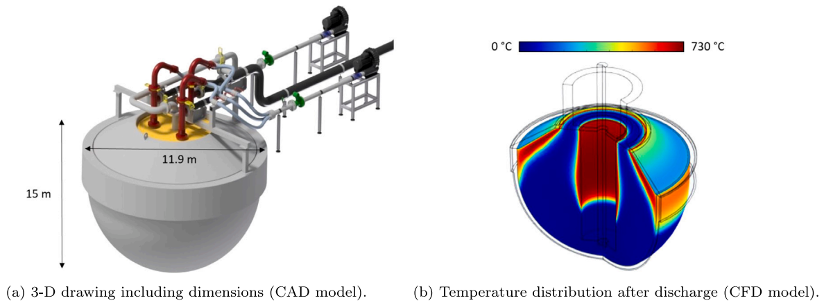
Fig. 2. Thermal energy storage module used in this work. Main parameters are provided in Table 2.
