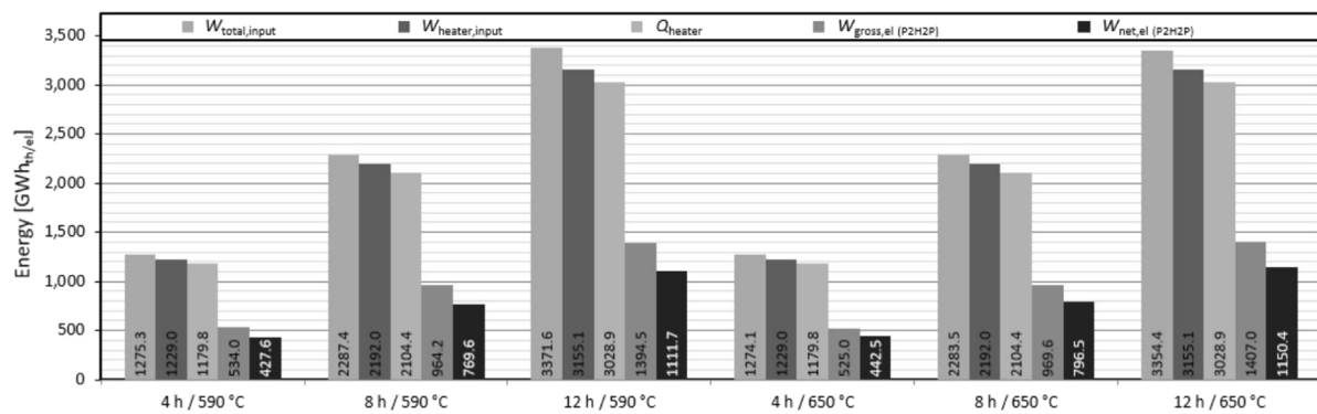
Fig. 6. Comparison of energies for all considered cases (all 10 h charge).
