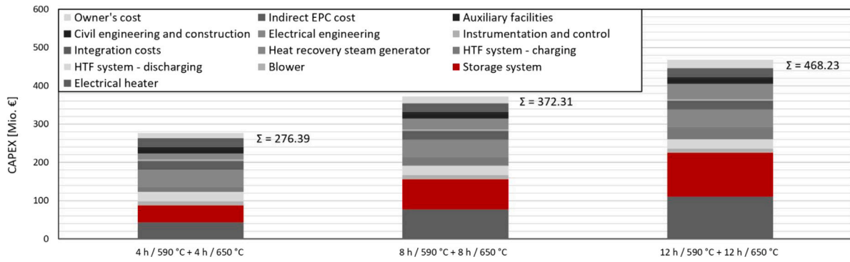
Fig. 9. CAPEX of all considered cases. The different categories are consistent with Table 4.
