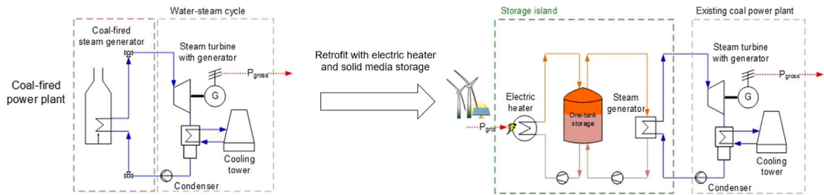
Fig. 1. Integration of a solid storage in retrofit concepts with electrical heater (adapted from [3,4]). Please note that a by-pass in the storage discharge circuit for the control of the steam generator inlet temperature is not depicted here for the sake of simplicity.
