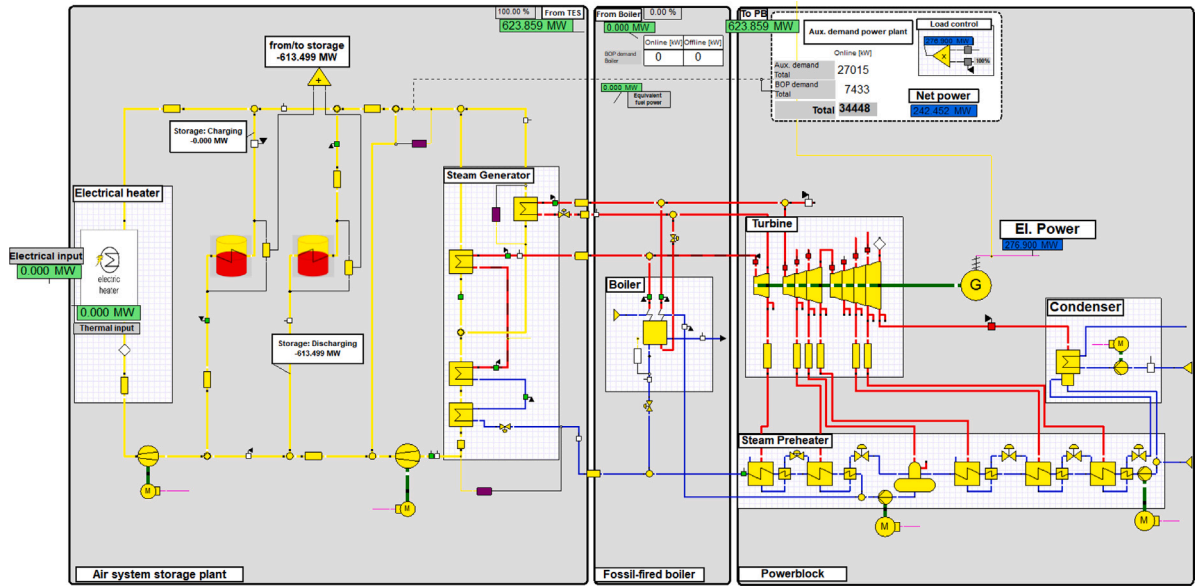
Fig. 5. Overview of the process simulation model for the discharging profile.
