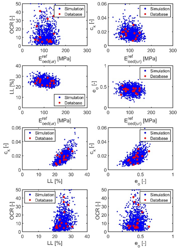
Figure 8. Comparison between the original database and 1000 simulated data based on multivariate model B.
