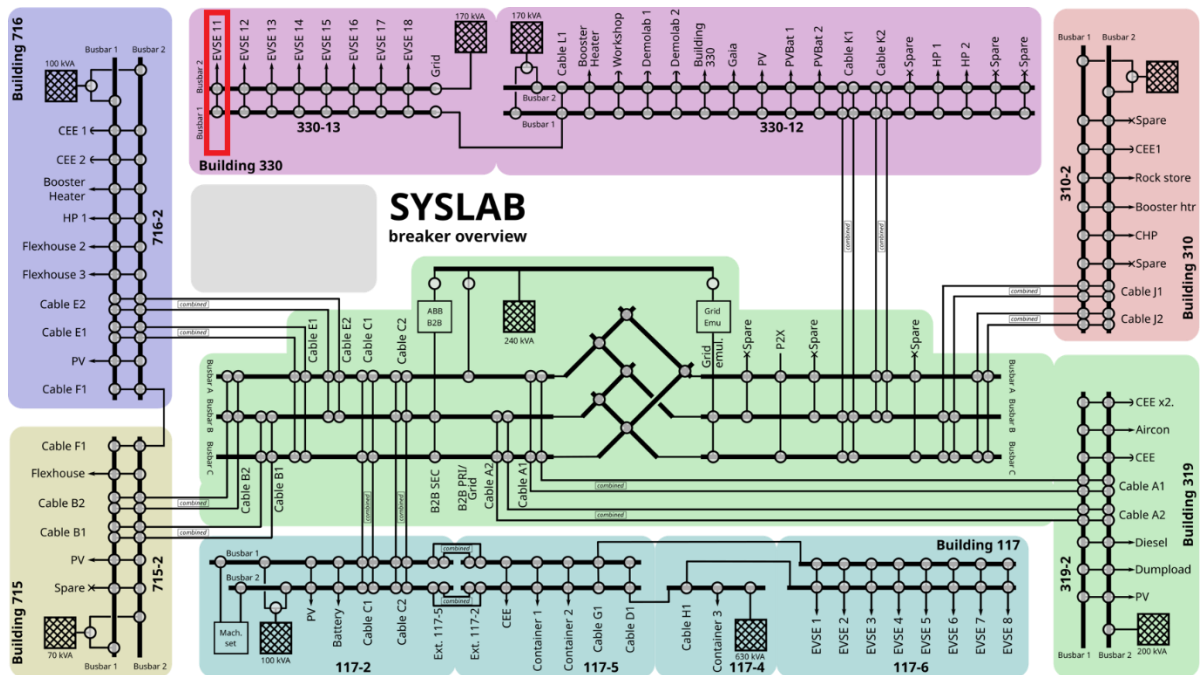
Figure 3: Schematic overview of the electrical SYSLAB nodes. The cluster connection point is highlighted as EVSE 11.
