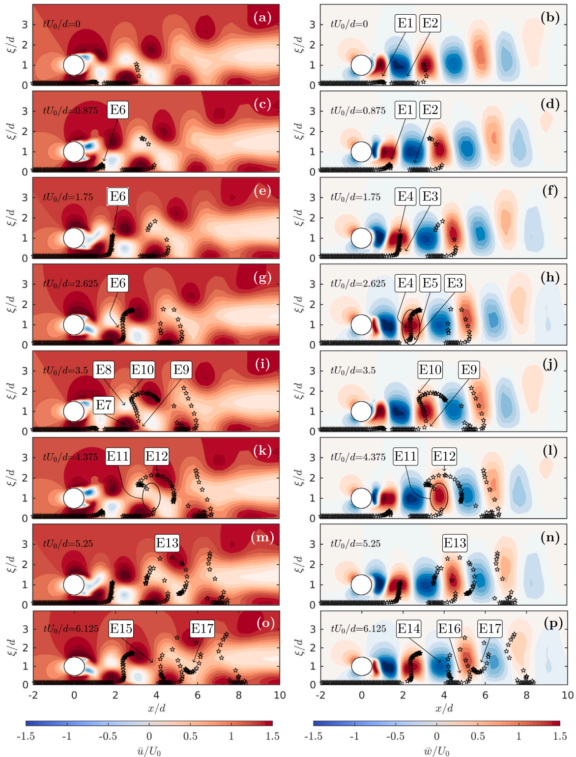
Fig. 5. Particle paths over two vortex shedding cycles. d = 0.08 m and e/d = 0.5 . Left: mean horizontal velocity component. Right: mean vertical velocity component. E1: Ejection. E2: No ejection. E3: Small mean vertical velocity. E4: High mean vertical velocity. E5: Vertical line of particles. E6: Mean horizontal velocity close to U_0 . E7: High mean horizontal velocity. E8: Low mean horizontal velocity. E9: Particles further downstream. E10: Particles further upstream. E11: Gap between particles. E12: Half-circle of particles. E13: Particles from half-circles spread out to zones with positive and negative mean vertical velocity. E14: Particles settling. E15: Large mean horizontal velocity. E16: Ejection. E17: Particles raise for the second time.
