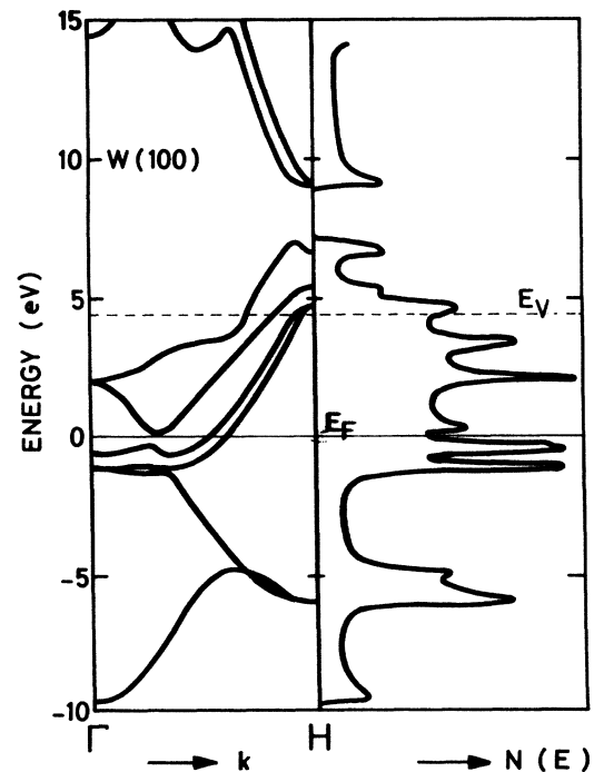
FIG. 5. Calculated band structure of tungsten along the \Gamma H symmetry line (left-hand side) and one-dimensional density of states (right-hand side).
