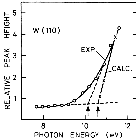
FIG. 14. Relative height of the leading peak in the spectra taken normal to the (110) face (peak A in Fig. 13) as a function of photon energy. Measured values, \circ ; calculated peak height, \times .
