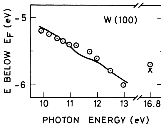
FIG. 8. Movement of initial-state energy of structure assigned to emission following direct optical excitation (peak C in Fig. 6) as a function of photon energy. Solid line and \times , calculated; \odot , measured peak position.
