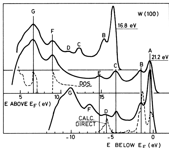
FIG. 10. Energy-distribution curves of photoelectrons emitted normal to the (100) face of tungsten for 16.8- and 21.2-eV photon energies. Top and bottom curve are identical (16.8 eV) but shifted horizontally such that the upper horizontal scale refers to final-state energy and the bottom scale refers to initial-state energy. The dashed lines give calculated curves for the density of states (DOS) or the contribution due to direct optical transitions (Calc. Direct) at 16.8-eV excitation energy.
