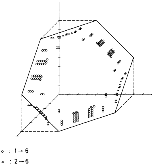
FIG. 16. Triangles indicate the loci of 2 → 6 transitions and circles correspond to 1 → 6 transitions of energy \hbar\omega = 10.2 eV and initial-state energy 4.16 eV below E_F .
