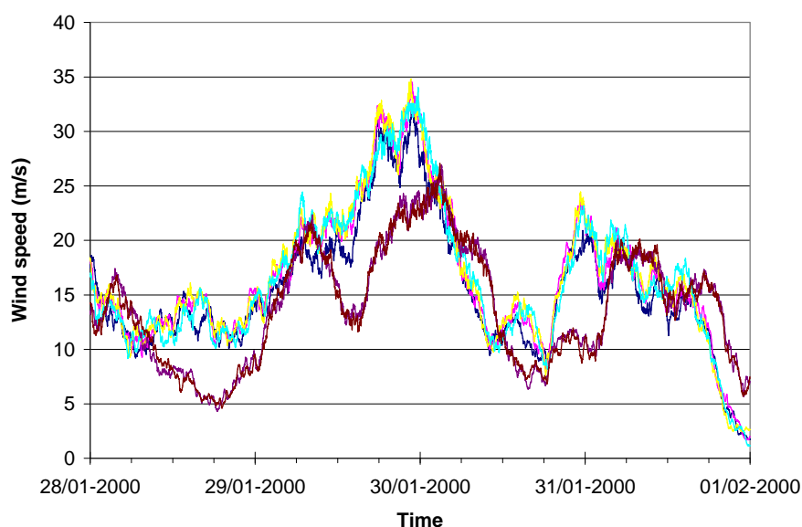
Figure 17. Wind farm averages of simulated wind speeds
