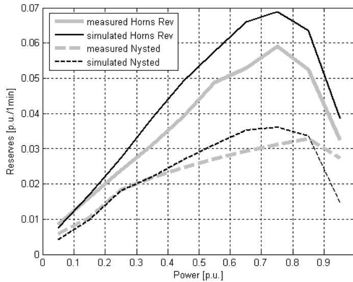
Figure 14. 1 % percentiles of 1 minutes reserve requirements in Horns Rev and Nysted wind farm
