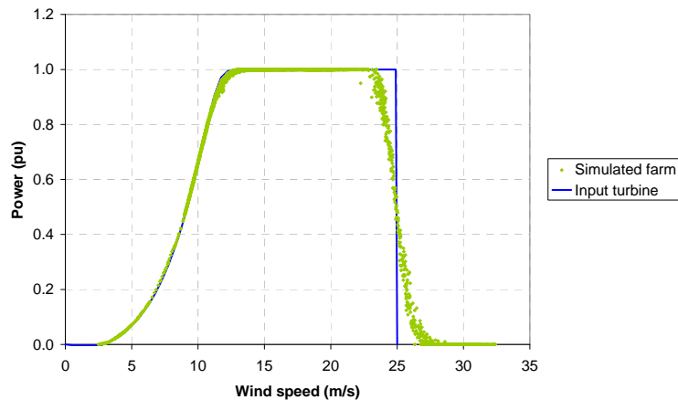
Figure 19. Simulated wind farm power curve compared to input power curve for wind turbine.
