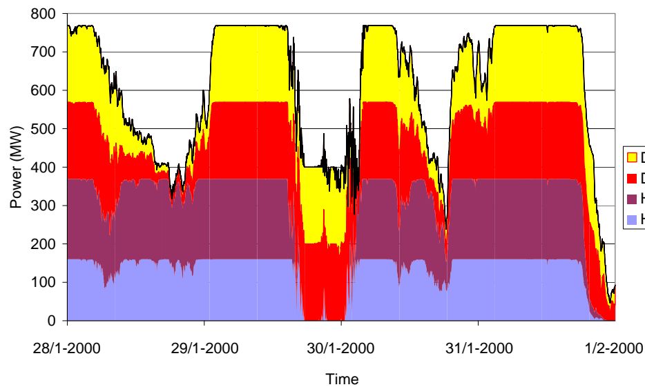
Figure 21. Simulated wind power fluctuations in the spread scenario
