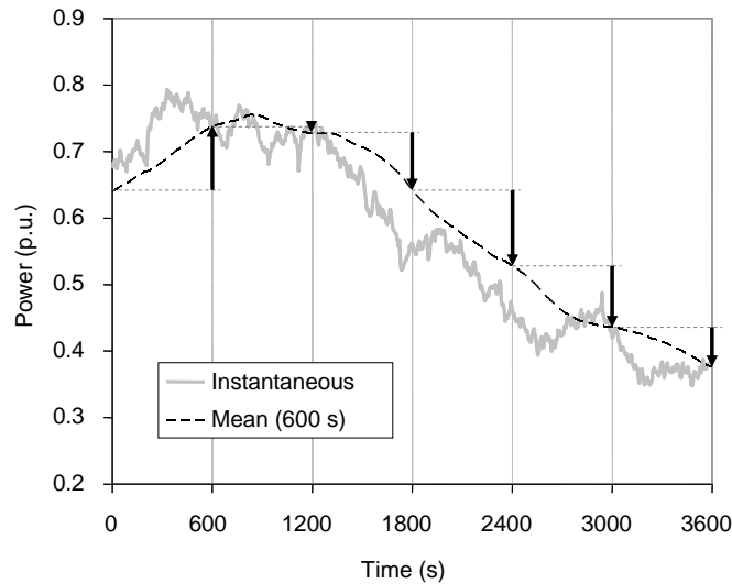
Figure 6. Definition of ramp rates for period time T_{\text{per}} = 10 min. The ramp rates are indicated with arrows.
