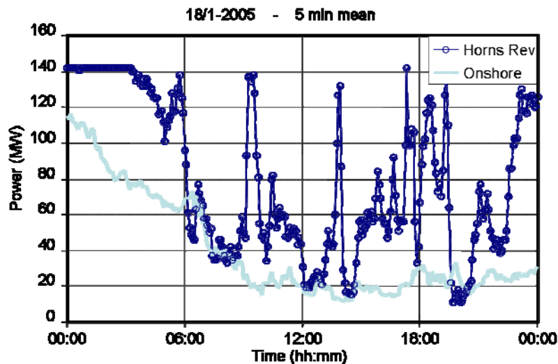
Figure 1. Power generation of Horns Rev offshore wind farm and onshore wind turbines January 18 2005.
