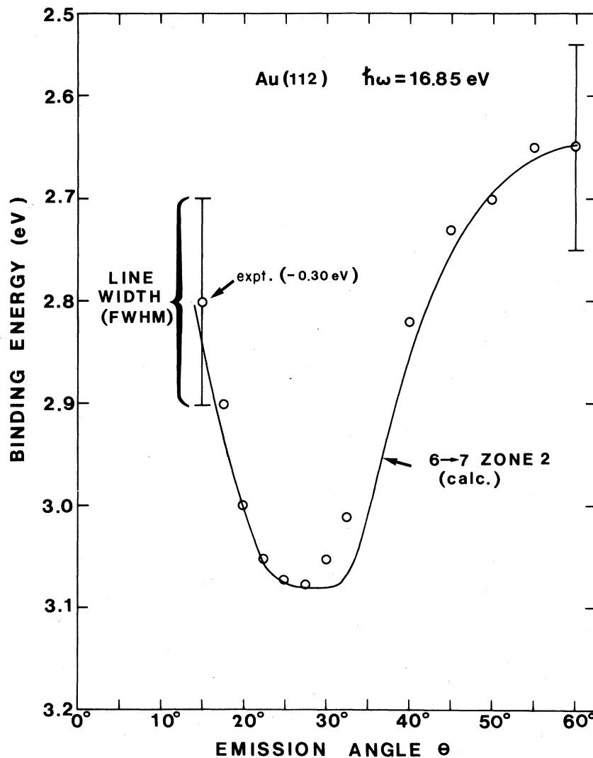
FIG. 2. Angular variation of the 6 \rightarrow 7 transition (full line) as calculated from the band model. The circles represent experimental (Ref. 8) peak positions (binding energies reduced by 0.30 eV). An estimate of the linewidth, full width at half maximum (FWHM), is indicated.
