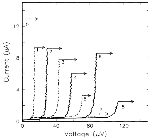
FIG. 2. Current vs voltage for various numbers of solitons at 4.2 K. Full curves: no solitons trapped. Dashed curves: one trapped soliton. The number next to each curve is the total number of solitons and antisolitons moving to produce that curve. The right-pointing arrows at the top of each curve mark the points at which the junction switches out of the various soliton branches. Junction parameters are J=67 A/cm 2 , \lambda_j=59 \mu m, L=875 \mu m, L/\lambda_j=14.8 , \alpha=0.018 , and \beta=0.01 .
