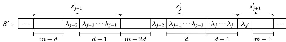
■ Figure 10 The structure of the j th sample in S' .
