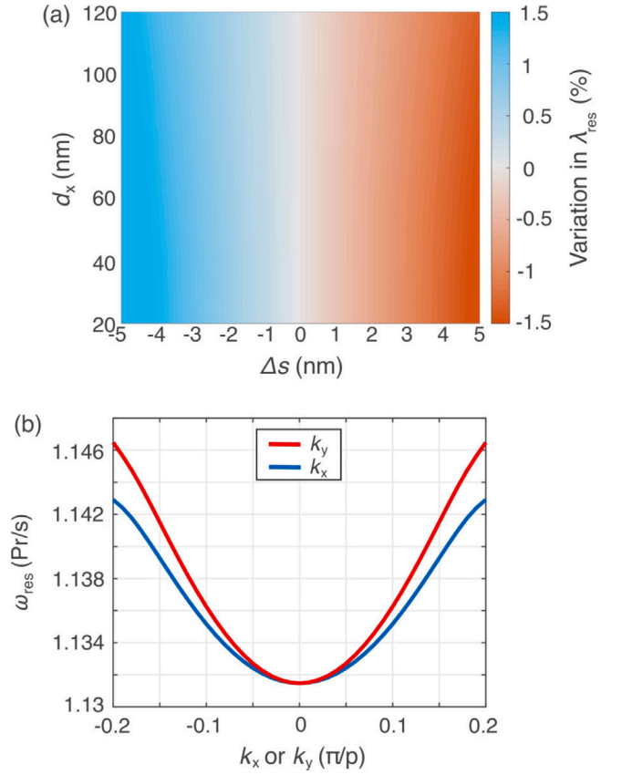
Fig. 6. (a) Variation of the qBIC resonant wavelength \lambda_{\text{res}} as a function of d_x and the slot width s = s_0 - \Delta s , where s_0 = 40 nm. (b) Angular dispersion of the qBIC mode for the symmetric metasurface.
