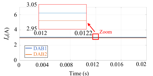
Fig. 7. Average output current using IPOP structure with leakage inductance L_1=50 \mu H, L_2=45 \mu H.
