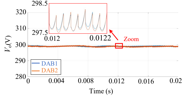
Fig. 5. Output voltage using IPOS structure with leakage inductance L_1=50 \mu H, L_2=45 \mu H.
