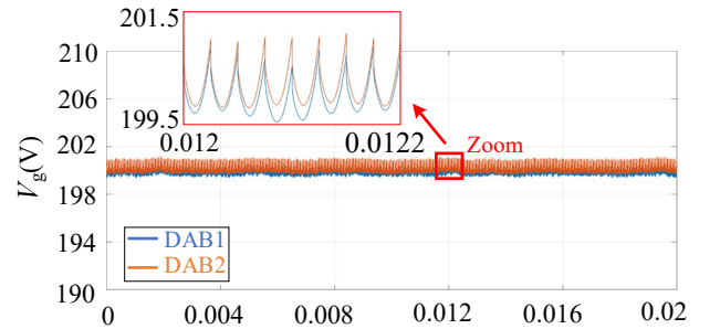
Fig. 6. Input voltage using ISOP structure with leakage inductance L_1=50 \mu H, L_2=45 \mu H.
