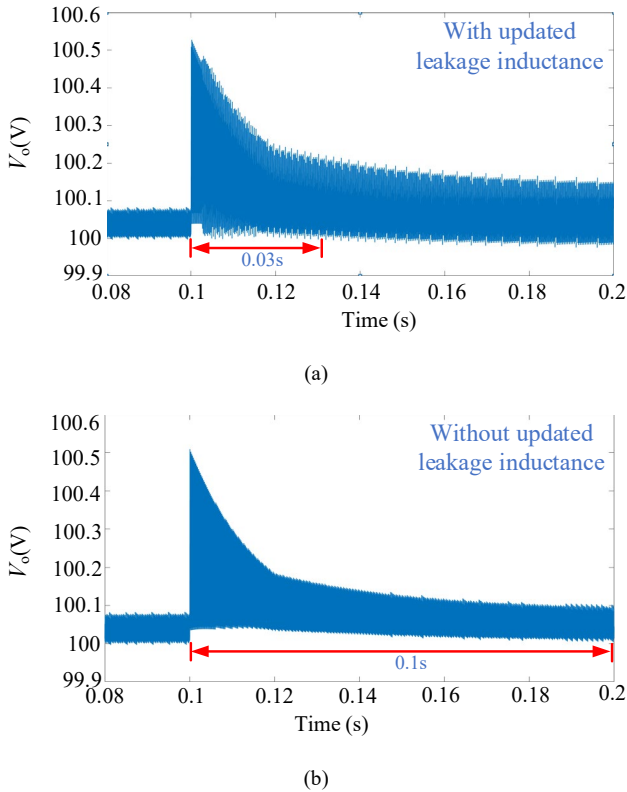
Fig. 3. Output voltage when leakage inductance change. (a) With the updated leakage inductance. (b) Without the updated leakage inductance.
