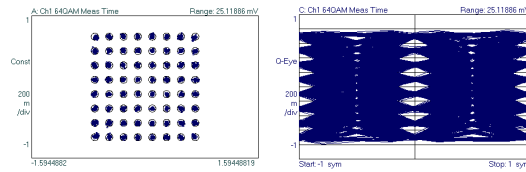
Figure 6: Output 64-QAM constellation (a, left) and Q symbol eye diagram (b, right).
