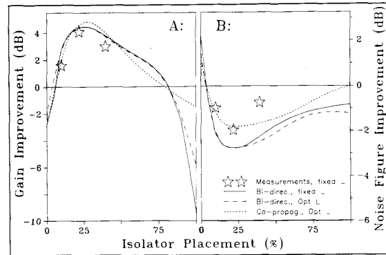
Fig. 3. (a) Gain versus relative isolator placement among 0 and 100% of the total fiber length. (b) Noise figure versus relative isolator placement. Measurements illustrated by stars. Calculations corresponding to the experiment are shown as solid lines. Calculations at gain optimized lengths in a bidirectional and copropagating pumping scheme are shown as dashed and dotted lines, respectively.
