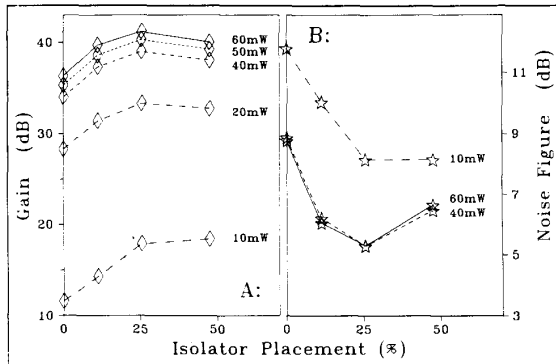
Fig. 2. Measured gain and noise figure versus the relative isolator placement between 0 and 50% of the total fiber length. Shown for pump power levels between 10 and 60 mW.
