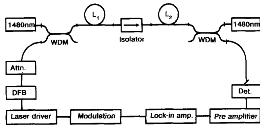
Fig. 1. Experimental setup. Not shown in the figure are monitor couplers at the signal input end of the two pump inputs.
