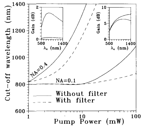
Fig. 1. Optimum cutoff wavelength versus pump power. The input signal power is -40 dBm. The left inset shows gain versus cutoff wavelength for a pump power of 1 mW, and the right for 100 mW. The upper lines are for NA = 0.4 and the lower for NA = 0.1. No filter is used in the insets.
