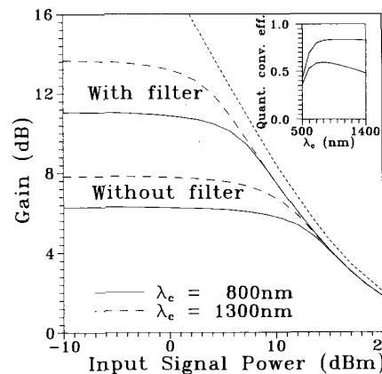
Fig. 2. Gain versus signal power for a pump power of 100 mW. The dotted line to the right is the theoretical limit, when the quantum conversion efficiency is 100%. The inset shows the quantum conversion efficiency versus cutoff wavelength.
