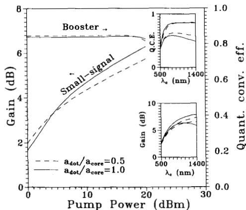
Fig. 3. Small-signal gain ( P_s = -40 dBm) and booster quantum conversion efficiency ( P_s = 15 dBm) versus pump power with 100% and 50% confinement of the Nd-doping. NA = 0.4, \lambda_c = 800 nm. The upper inset shows booster quantum conversion efficiency versus \lambda_c , the lower inset shows small-signal gain versus \lambda_c , both for 100 mW of pump power, and NA = 0.4 and NA = 0.1.
