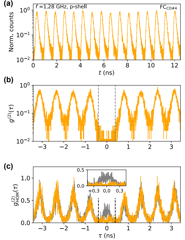
Figure 5: Performance of the fiber-pigtailed QD device ( X^+ emission) under p-shell excitation at a clock-rate of f=1.28 GHz. The temporal delay between consecutive single-photon amounts to 1/f = 781 ps. (a) Time-resolved trace of a single-photon pulse train in logarithmic scaling. (b) Photon-autocorrelation g^{(2)}(\tau) -measurement. (c) Two-photon interference g_{\text{HOM}}^{(2)}(t) histograms measured in co- (orange) and cross- (grey) polarized configuration at P_{\text{exc}}=P_{\text{sat}}/16 . Dashed lines indicate the 781 ps repetition period.
