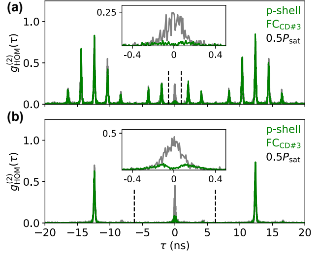
Figure 4: Two-photon interference measurements for the FC-device. The g_{\text{HOM}}^{(2)}(\tau) measurements were taken during FC CD#3 under 80 MHz p-shell excitation at half the saturation power P_{\text{sat}} . Co-polarized measurements are shown in green, cross-polarized measurements in grey. (a) For a separation of \delta t = 2 ns for the exciting pulses. (b) For a separation of \delta t = 12.5 ns for the exciting pulses. The HOM visibility V_{\text{HOM}} is obtained by comparing the co- and cross polarized peak areas at \tau = 0 . The respective integration time-windows are indicated with dashed lines.
