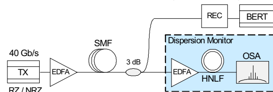
Figure 2 : Setup used to perform dispersion monitoring on 40 Gb/s RZ or NRZ signals.
