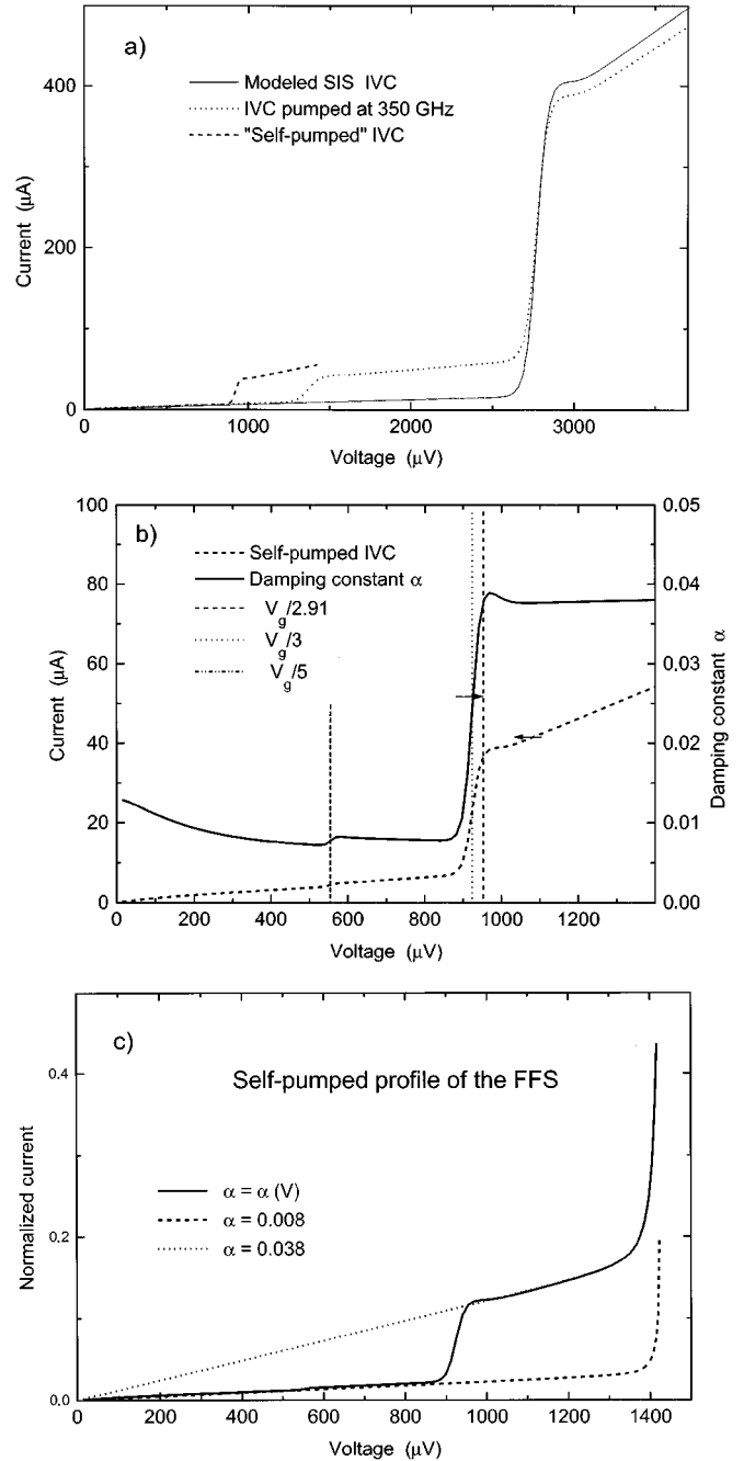
FIG. 4. (a) Modeled SIS I - V characteristics: autonomous (solid line), and pumped at f = 350 GHz (dotted line). The “self-pumped” I - V characteristics are shown by the dashed curve. (b) “Self-pumped” I - V characteristics (dashed line) and damping constant \alpha_k (solid curve); see text. (c) Calculated profile of the FFS for the voltage-dependent damping \alpha_k(V_k) , solid curve. The FFS profiles at fixed \alpha values 0.008 and 0.038 are shown by dotted and dashed lines, respectively.
