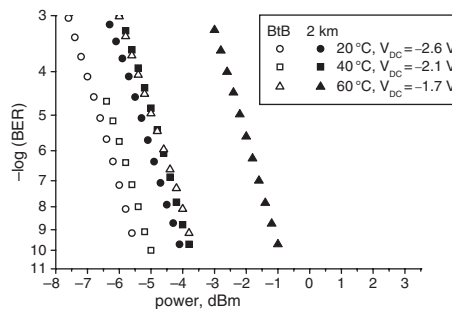
Fig. 1 BER dependence on temperature for uncompensated system
