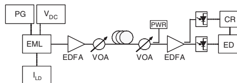
Fig. 2 Schematic for compensated transmission
