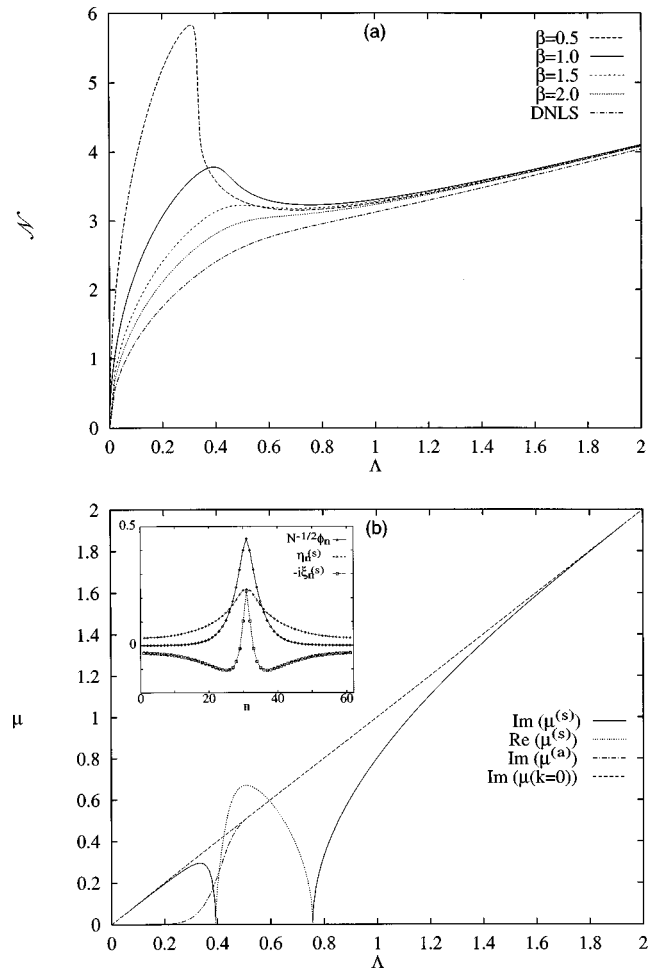
FIG. 1. (a) Dependence \mathcal{N}(\Lambda) for stationary on-site localized solutions to Eq. (1) with J_n exponentially decreasing. From top to bottom in the left part of the figure, \beta=0.5 , \beta=1.0 , \beta=1.5 , \beta=2.0 , and \beta \rightarrow \infty , respectively. (b) Eigenvalues \mu of the matrix \mathcal{M} in Eq. (2) versus \Lambda for \beta=1.0 . The solid (dotted) line shows the imaginary (real) part of the eigenvalue \mu^{(s)} corresponding to the spatially symmetric, localized mode; the dash-dotted line shows the imaginary part of the eigenvalue \mu^{(a)} corresponding to the translational mode; the straight dashed line shows the lower bound of the continuous spectrum. (The spectrum is symmetric around \mu=0 .) The inset in (b) shows, from top to bottom at n=n_0=31 , \phi_n/\sqrt{\mathcal{N}} , \eta_n^{(s)} , and -i\xi_n^{(s)} , respectively, where \phi_n is the stationary state used as the initial condition in Fig. 2(a) and (\xi_n^{(s)}, \eta_n^{(s)})^T is the corresponding normalized eigenvector of the matrix \mathcal{M} with eigenvalue \mu^{(s)} \approx 0.286i (choosing the overall phase so that \eta_n^{(s)} is real and positive).
