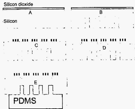
Figure 4: Fabrication sequence for the flexible silicon stamp. The final flexible stamp is a hybrid between silicon and PDMS. All the silicon processing is performed by bulk silicon micro machining which is followed by molding of the PDMS mattress to the back side.
