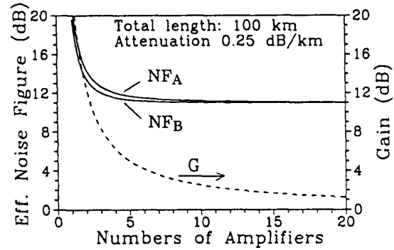
Fig. 2. Effective noise figures NFA and NFB for the power and preamplifier configuration respectively, versus the number of amplifiers within a 100 km fiber span. The dashed curve display the gain G of each amplifier.
