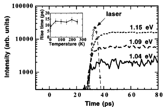
FIG. 4. PL rise dynamics at detection energies corresponding to the three lowest energy states in the QDs at 5 K and under strong excitation ( I_{\text{pump}}=300 \text{ W/cm}^2 , E_{\text{pump}}=1.55 \text{ eV} , detection energy window=40 meV). The dashed line represents the scattered pump laser pulse. Inset: Ground state rise time vs temperature ( I_{\text{pump}}=300 \text{ W/cm}^2 ).
