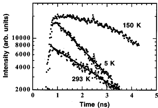
FIG. 2. Time-resolved PL decays as detected at the QD ground state for each temperature (average I_{\text{pump}}=9.4 \text{ W/cm}^2 , E_{\text{pump}}=1.55 \text{ eV} , detection window=10 meV). The continuous lines show monoexponential fits.
