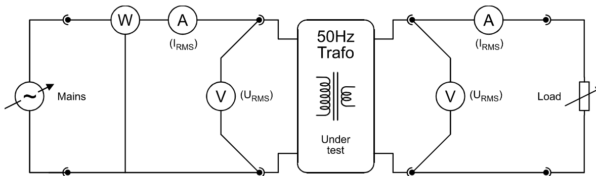
Figure 1 The Transformer Test Circuit
