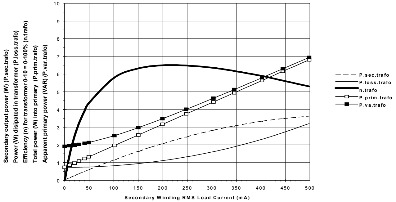
Figure 2 TR#1: A off-the-shelf transformer intended for a 5V-DC@1W series regulated power supply
