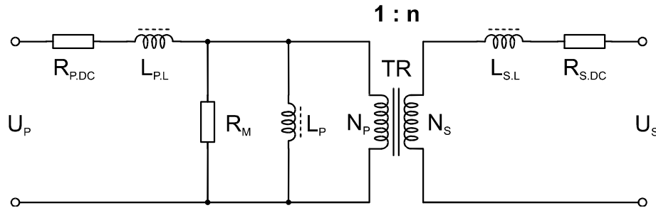
Figure 7 The Overall Transformer Equivalent Circuit
