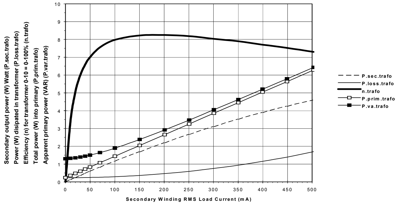
Figure 5 TR#4: The optimized transformer intended for a 5V-DC@1W buck based power supply
