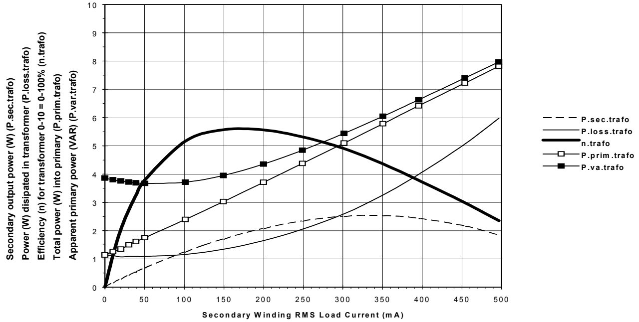
Figure 4 TR#3: The off-the-shelf transformer intended for a 5V-DC@1W buck based power supply
