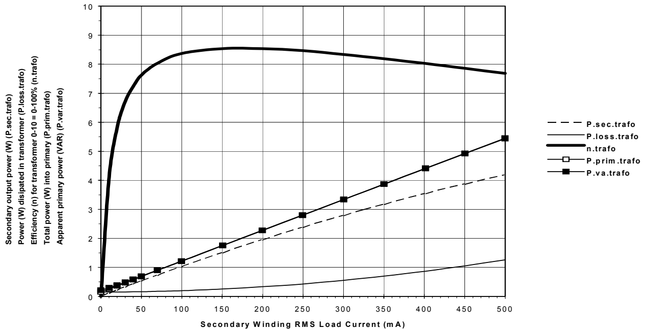
Figure 3 TR#2: The optimized transformer intended for a 5V-DC@1W series regulated power supply
