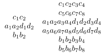
Fig. 2. Four 1 \times 2 blocks ( J = K = 1 ) and four blocks with J = K = 2 .
