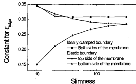
Figure 3: Value of the linear constant for \epsilon_{edge} as a function of the slinness, for 3 different scenarios: Ideally clamped boundary (squares), elastic boundary at the frontside (circles) and at the backside (triangles) of the membrane.
