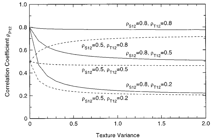
Fig. 6. The observed power correlation coefficient \rho_{P12} as a function of the texture variance \sigma_T^2 , for different combinations of \rho_{S12} and \rho_{T12} . The curves were evaluated using (5) assuming that the number of looks is L = 11 , \sigma_{T1} = \sigma_{T2} , and the SNR is large.
