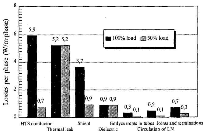
Fig. 4. Distribution of losses in a single-core HTS cable at 100% load and 50% load. The losses are distributed according to the components origin and the efficiency of the cooling machines is included in the values.
