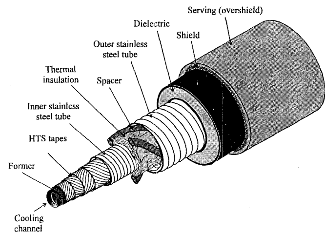
Fig. 1. Conceptual design of an HTS single-core power transmission cable used for the case study (room temperature dielectric design concept).
