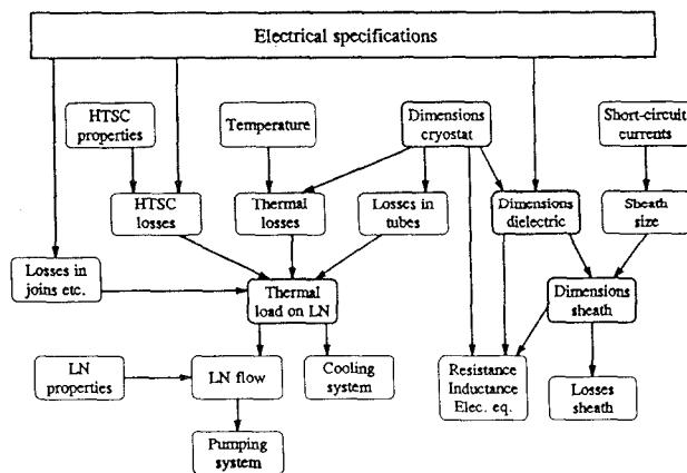
Fig. 2. Flow chart of calculation procedure of HTS cable.
