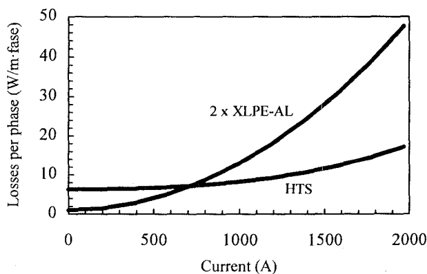
Fig. 3. Losses in 450 MVA HTS and conventional cable systems. The losses in the HTS cable system are smaller than the losses in the conventional cable system at high currents only.
