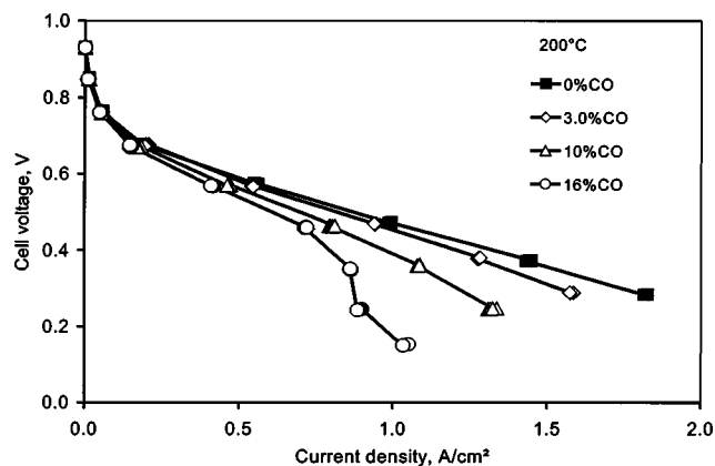
Figure 5. Polarization curves of a PBI-based PEMFC with pure hydrogen and hydrogen containing CO at 200°C. The CO concentrations are indicated in the figure.
