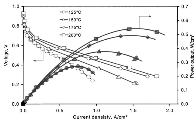
Figure 1. Polarization curves of a PBI-based PEMFCs at different temperatures. The working area of the electrodes was 10 \text{ cm}^2 . The PBI membrane was doped with 5.3 mol \text{H}_3\text{PO}_4 per repeat unit of the polymer. Oxygen and hydrogen were under atmospheric pressure. Hydrogen flow rate 27 \text{ mL min}^{-1} \text{ cm}^{-2} . Both anode and cathode were made of carbon-supported platinum catalysts (20% Pt/C) with a platinum loading of 0.5 \text{ mg Pt/cm}^2 . These parameters apply also to the following figures.
